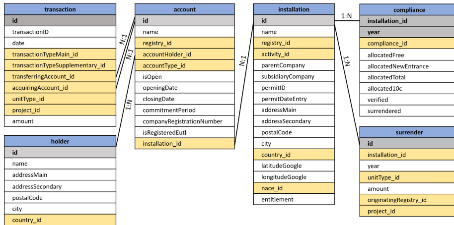
FIGURE 2. Relations in the EUTL Database
